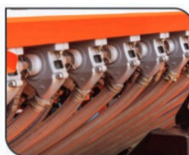
Seed Drill Feeder
